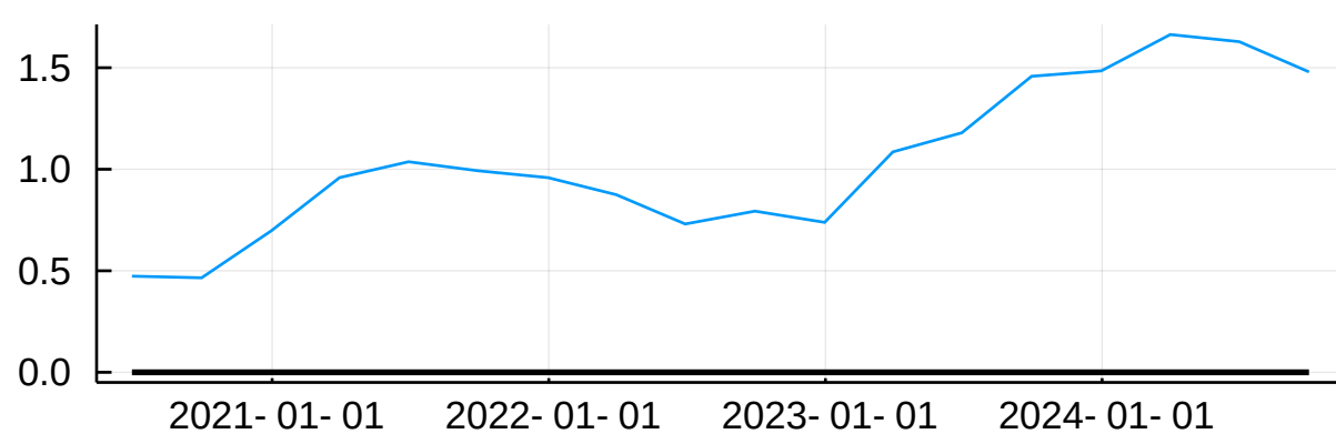
Real natural rate
