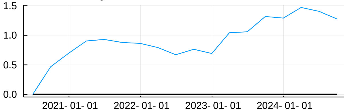
Change in r^* since end of COVID19
