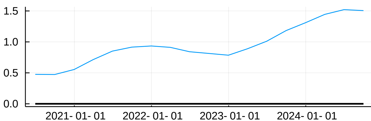
Ex- ante real rate
